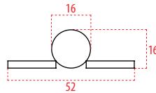
Sürgü Kapı Klavuz Rayı-4 Sliding Gate Track-4 (radius curved)
