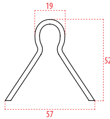
Sürgü Kapı Klavuz Rayı-3 Sliding Gate Track-3 (cement fixing)
